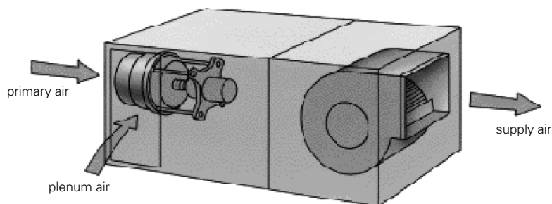
Figure 3—Series Fan-Powered VAV Terminal
