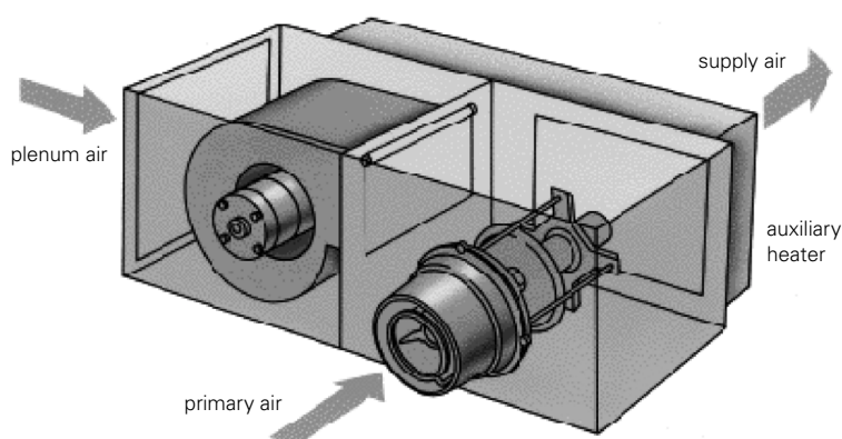
Figure 4—Parallel Fan-Powered VAV Terminal
